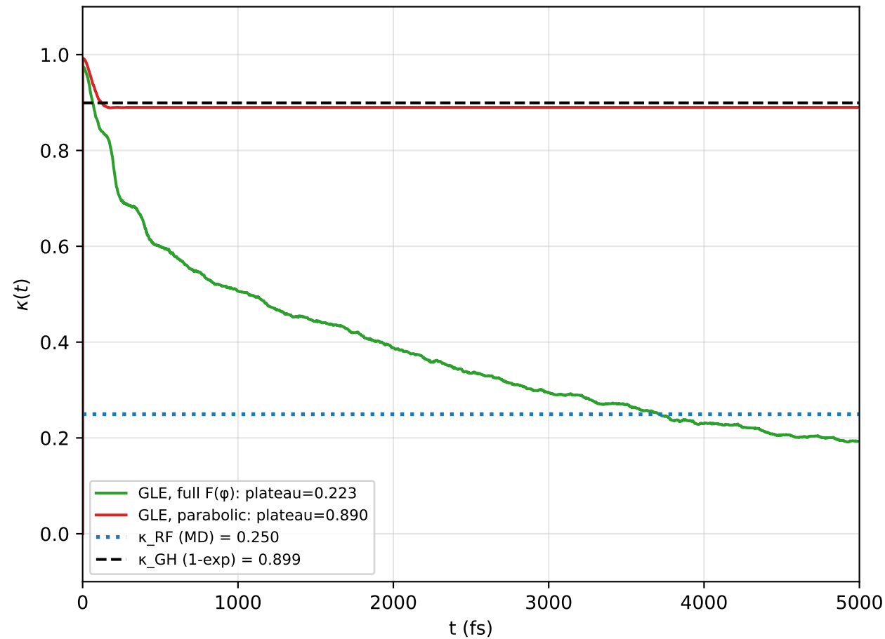
Butane GLE \kappa(t) : anharm vs harm (N=5000)
