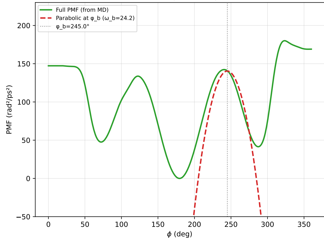
Anharmonic vs parabolic potential
