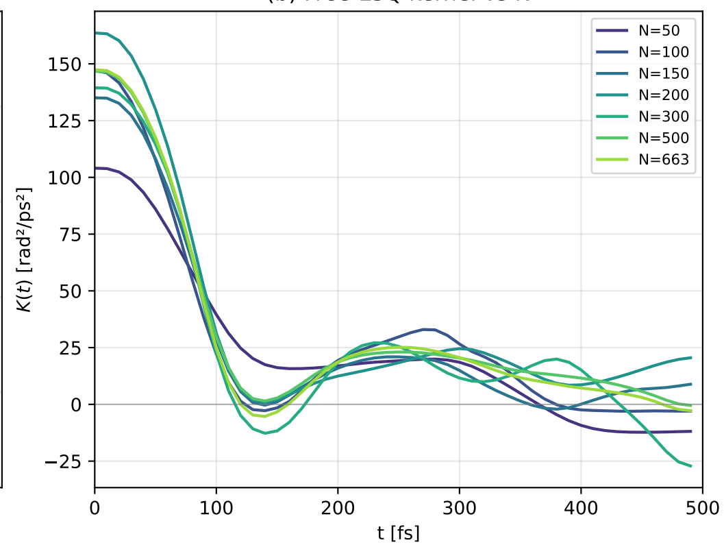
(b) Free-LSQ kernel vs N
