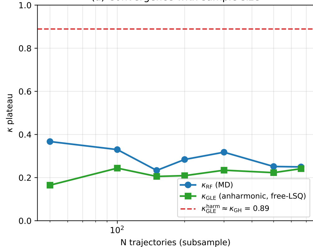
(a) Convergence with sample size
