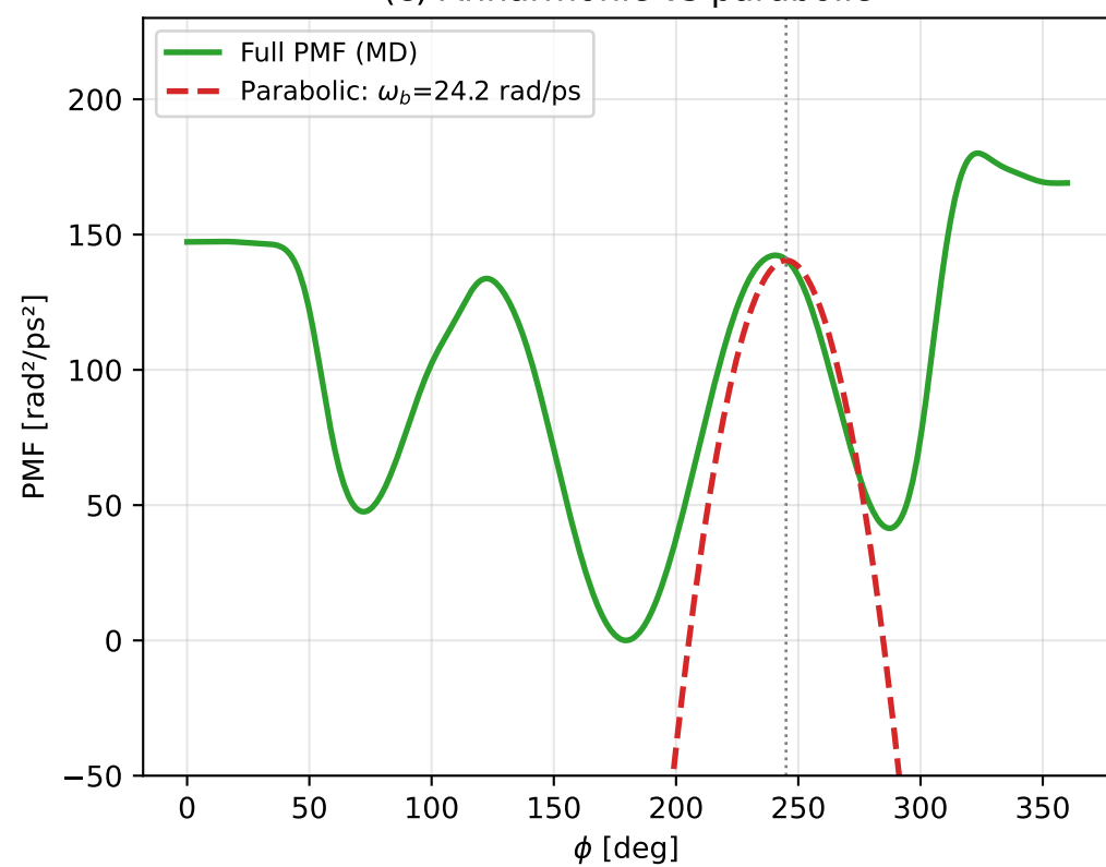
(c) Anharmonic vs parabolic
