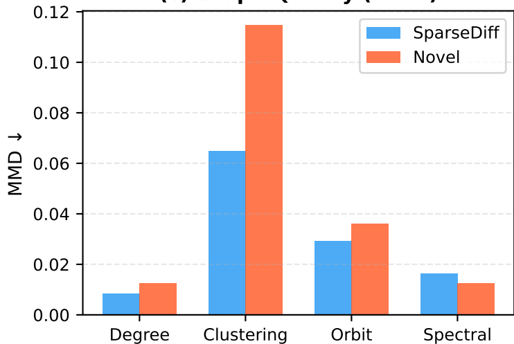
(c) Graph Quality (MMD)
