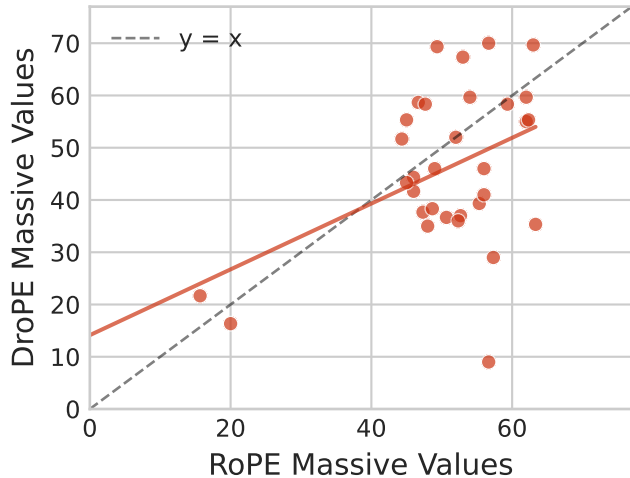
Key ( r = 0.43 )
