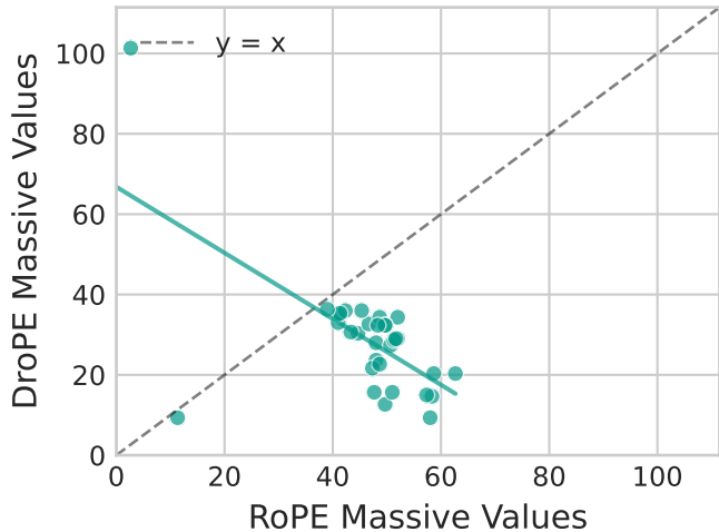
Query ( r = -0.62 )
