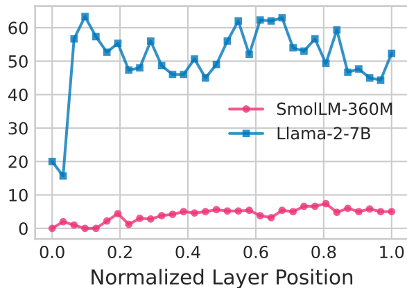
Key (K)
