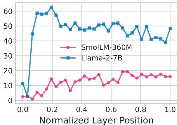
Query (Q)
