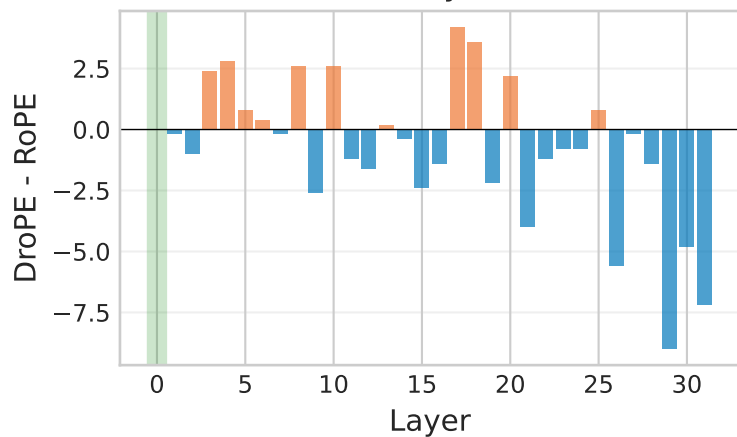
Query \Delta
