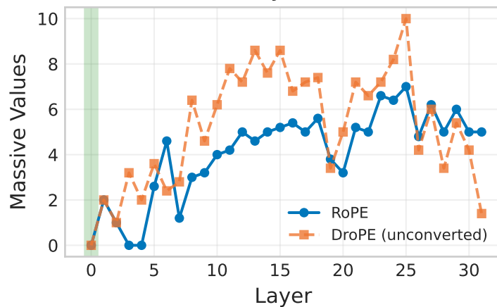
Key (K)
