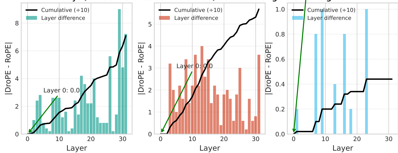
SmolLM: How Differences Accumulate Through Layers Layer 0 ~ 0 difference confirms massive values originate in weights
