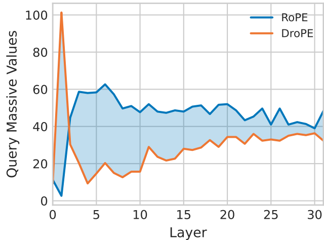
D. Reliance on Massive Values
