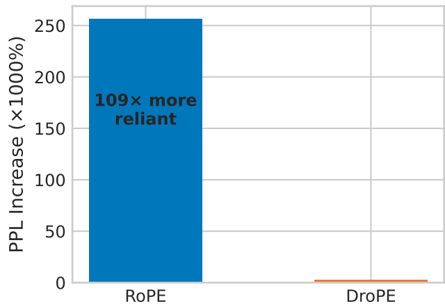
D. Reliance on Massive Values
