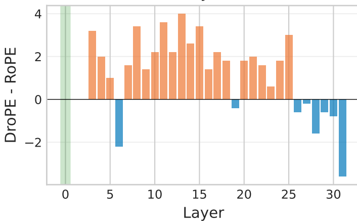
Key \Delta
