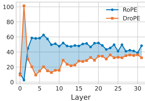
Query (Q)
