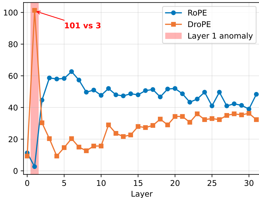
A. Layer 1 Anomaly: DroPE has 37x more
