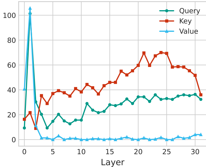
Llama-2-7B with DroPE
