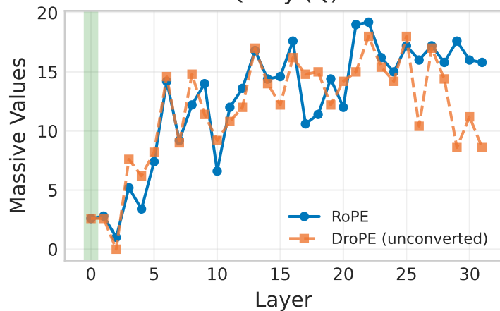
Query \Delta
