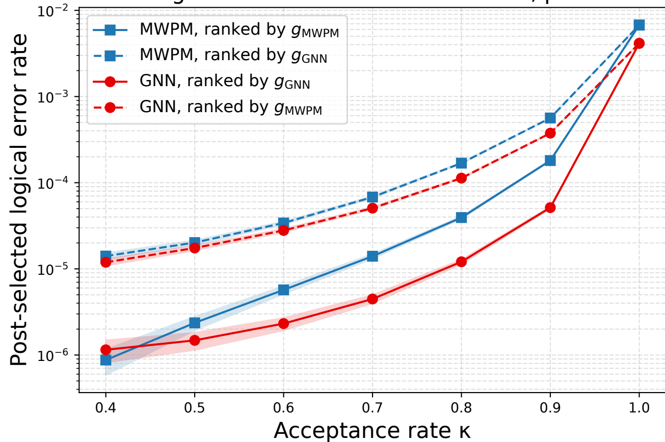
Exchanged confidence scores: d = r = 9 , p = 0.005
