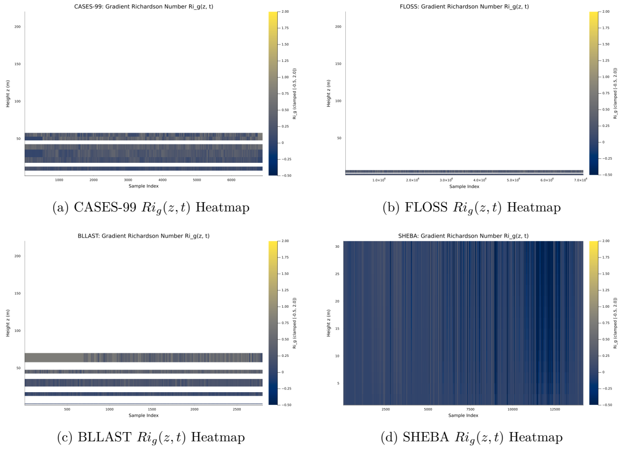
Figure 5: Gradient Richardson number time-height cross sections displaying boundary layer stability transitions across all four observational campaigns.
