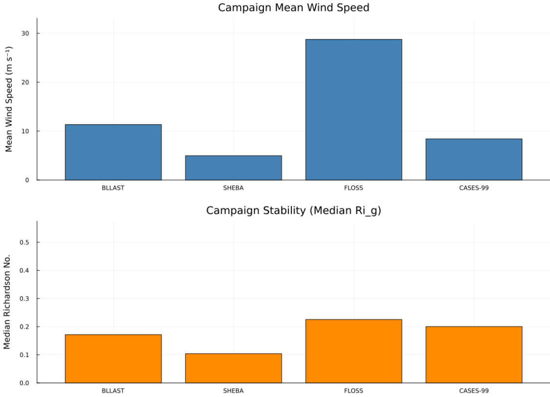
Figure 1: Comparative campaign overview displaying mean wind speed and stability metric profiles across all field sites.
