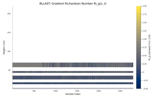
(c) BLLAST Ri_g(z, t) Heatmap
