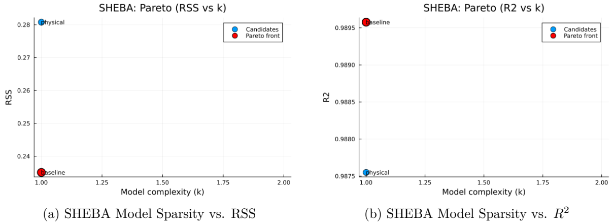
Figure 8: Pareto trade-off frontiers between closure complexity ( k ) and goodness-of-fit metrics for SHEBA.
