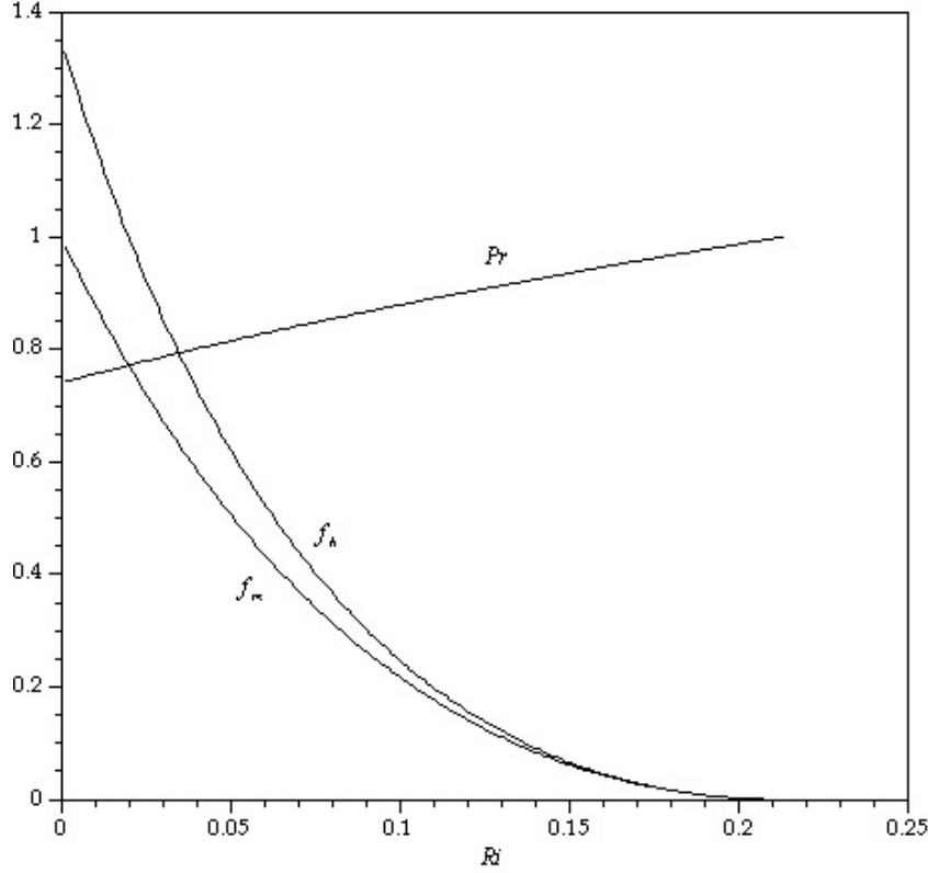
Figure 1: Stability functions for the stable boundary based upon the profiles (5).
