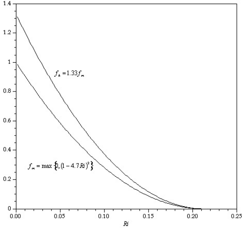
Figure 4: Approximate stability functions for the stable boundary layer.
