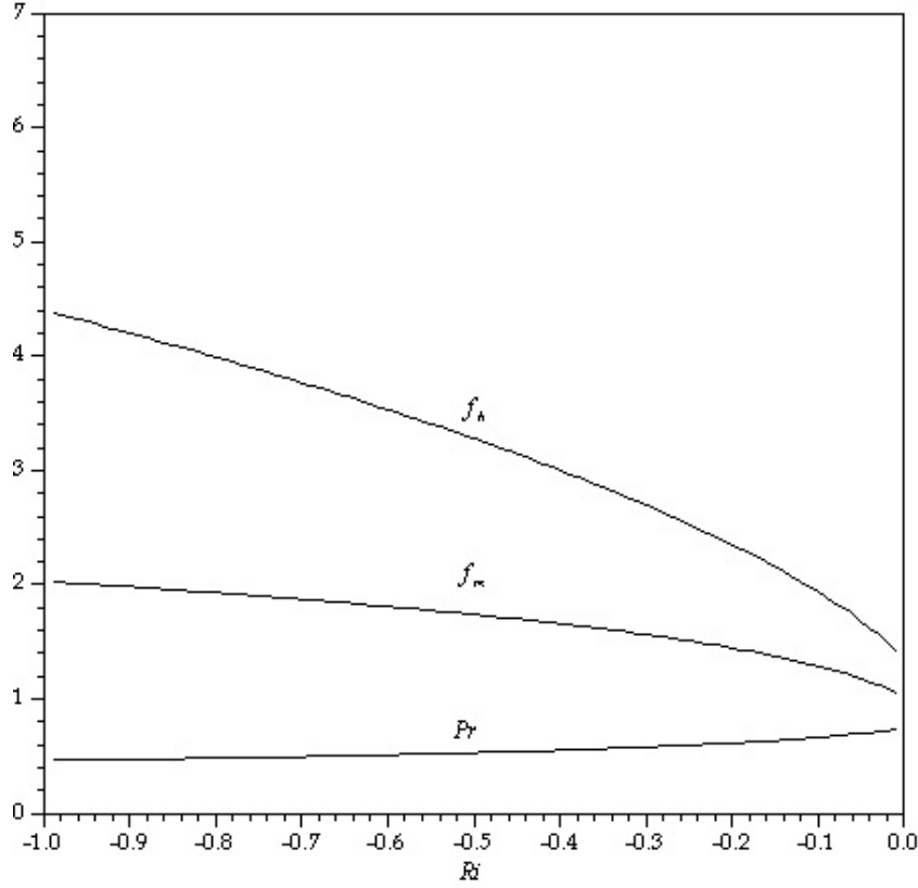
Figure 2: Stability functions for the unstable boundary based upon the profiles (??).
