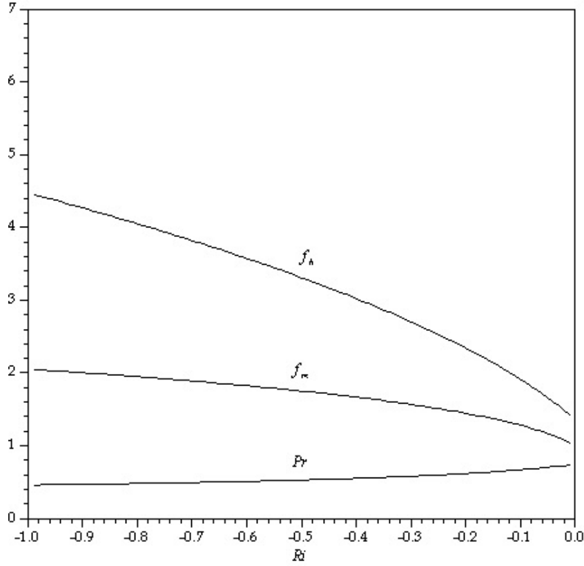
Figure 3: Approximate stability functions for the unstable boundary.
