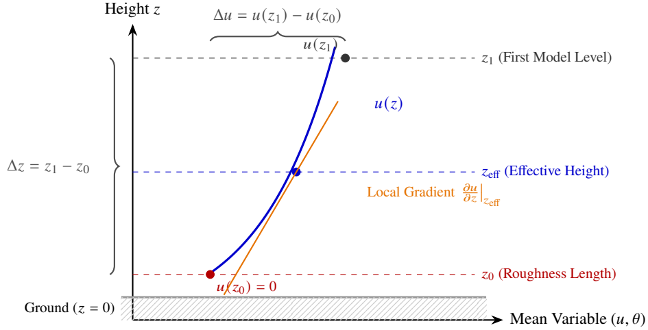
Figure 1: Schematic of discrete surface layer discretization illustrating the bulk layer differences over \Delta z and the effective height z_{\text{eff}} matching the local point gradient Ri_g to the bulk layer Ri_b .
