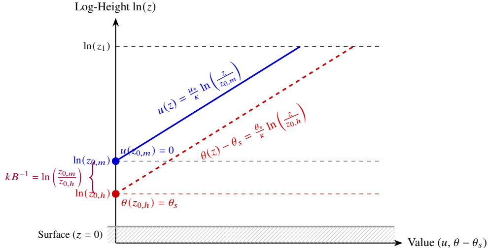
Figure 4: Neutral vertical profiles of wind velocity u(z) and potential temperature deviation \theta(z) - \theta_s plotted against logarithmic height \ln(z) . The logarithmic intercepts define z_{0,m} (where wind vanishes) and z_{0,h} (where atmospheric temperature matches ground skin temperature).
