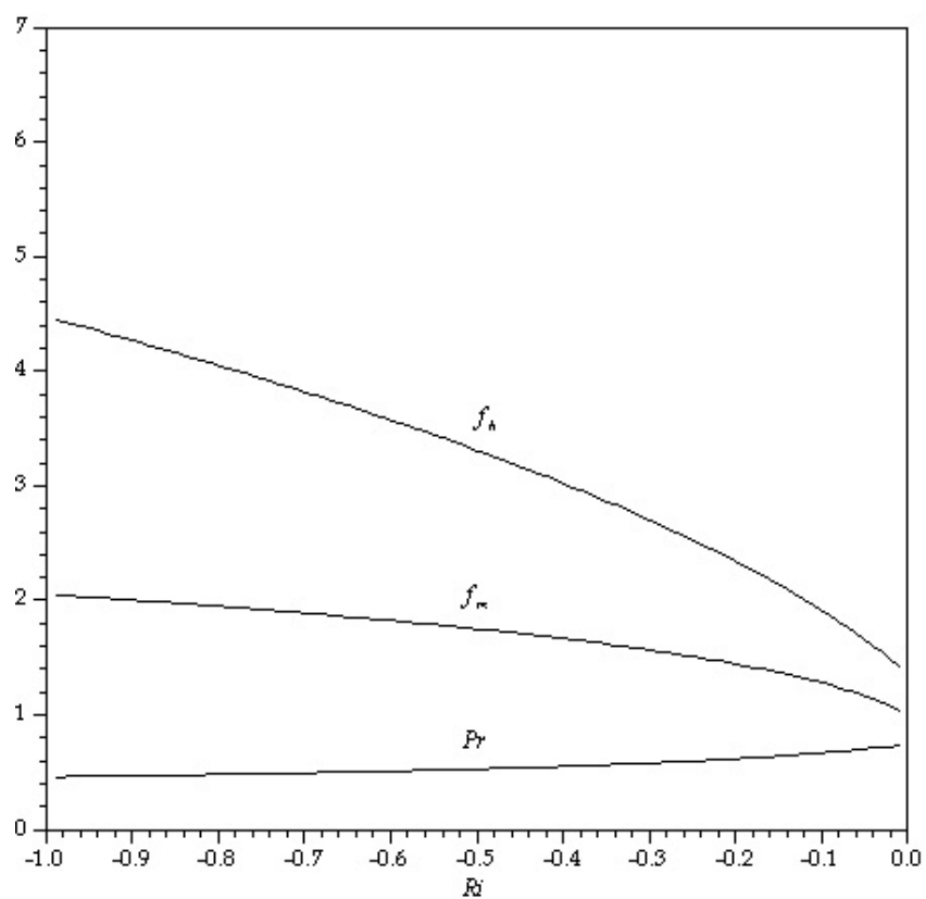
Figure 4: Approximate stability functions in the unstable boundary layer compared against exact solutions.
