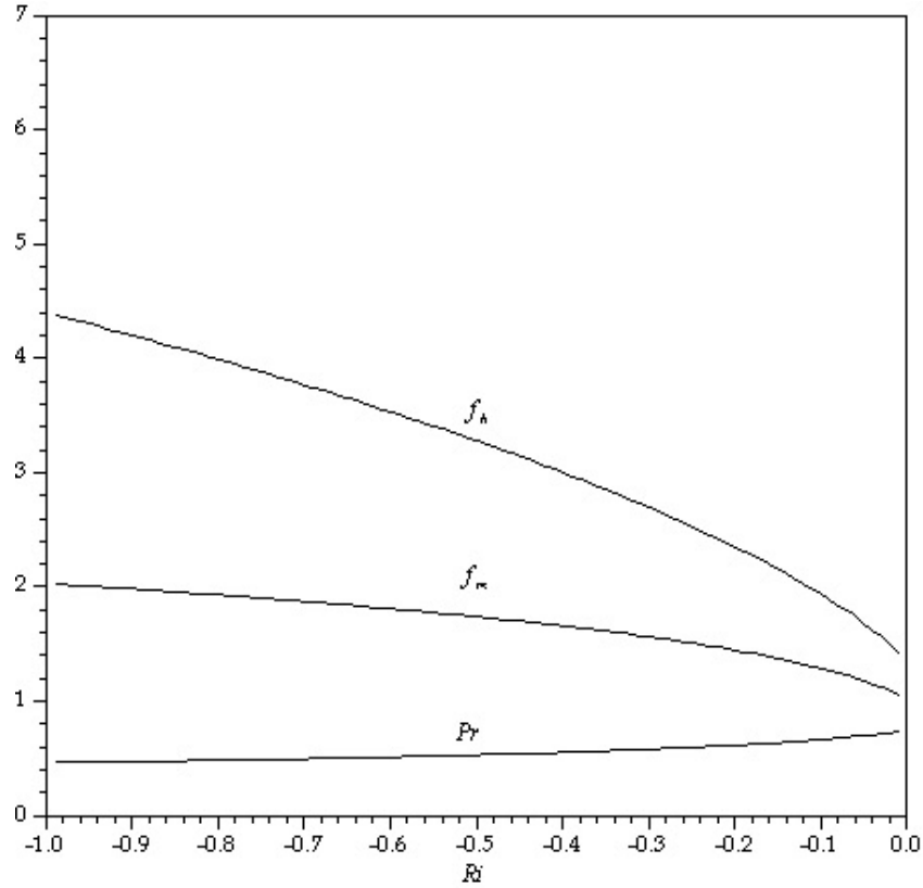
Figure 3: Exact stability functions f_m(Ri) , f_h(Ri) , and Prandtl number Pr(Ri) in the unstable boundary layer.
