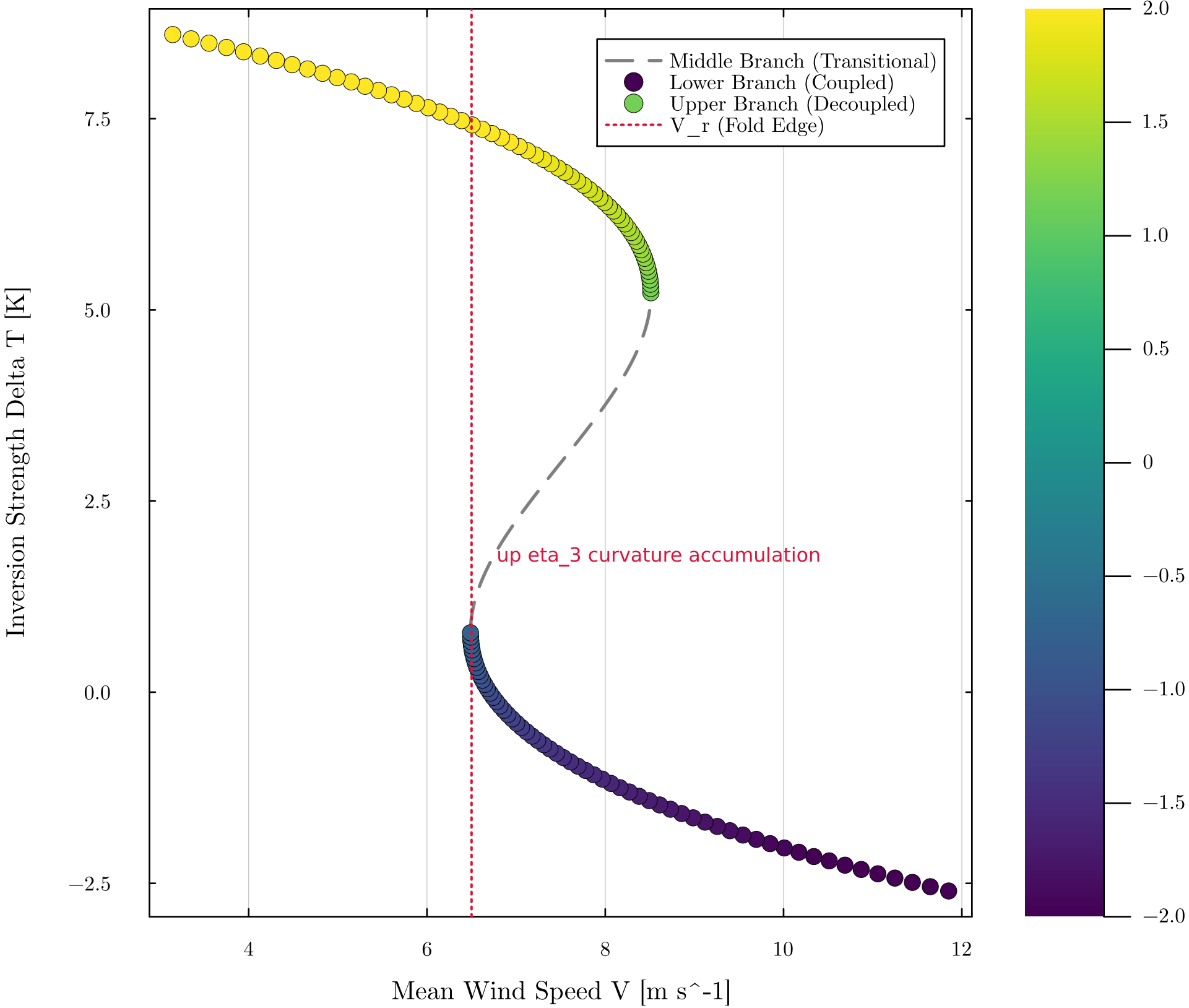
(a) CASES-99 / Santa Maria (Brittle Archetype)
