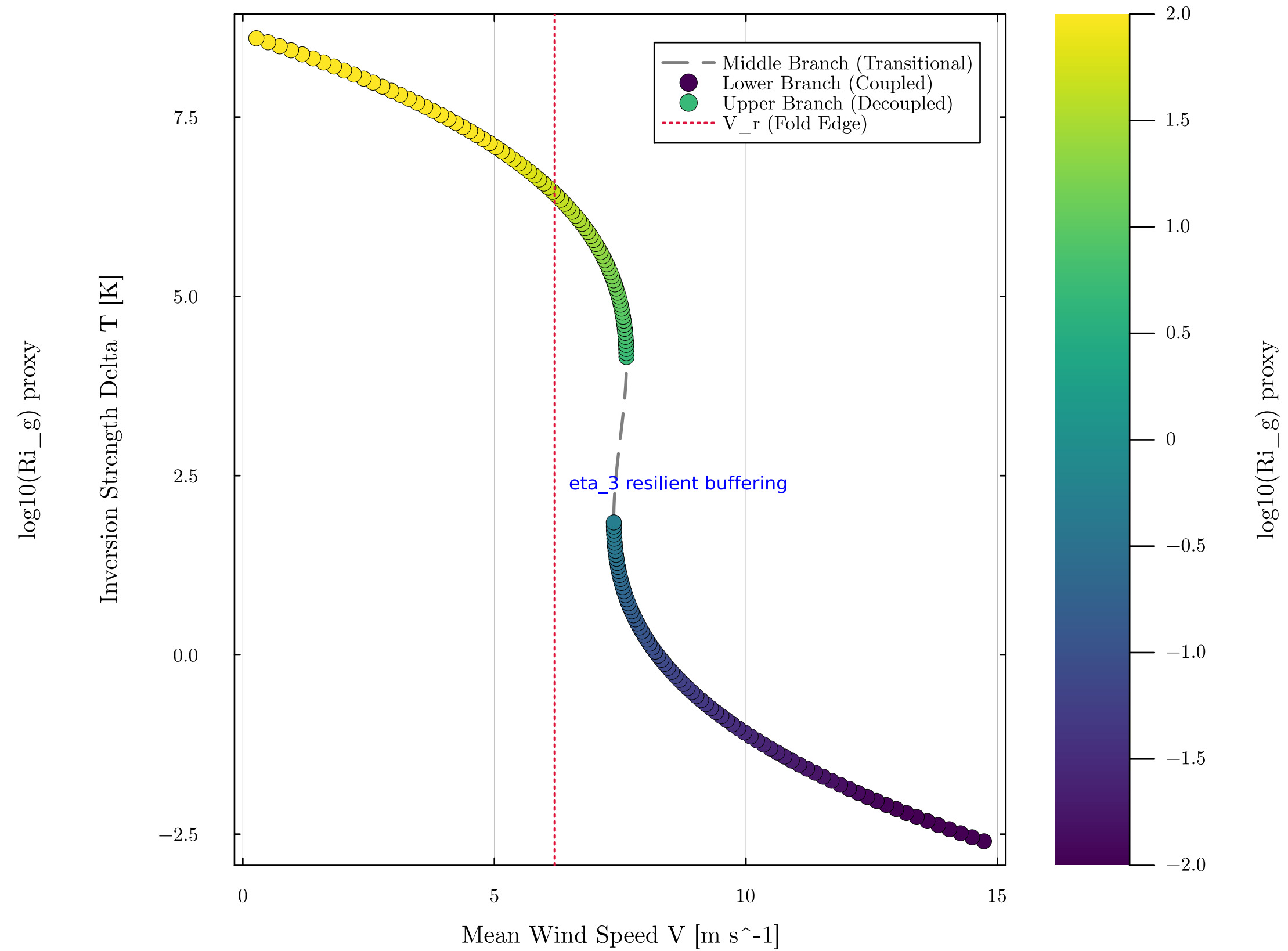
(b) FLOSS II / Polar Test (Rubbery Archetype)
