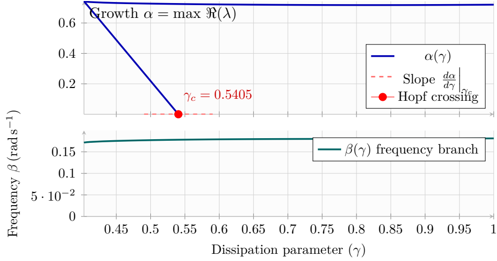
Figure 5: Stage 5 parameter continuation spectrum: the top panel charts the principal manifold stability branch \alpha(\gamma) , while the bottom panel shows the aligned oscillation-frequency branch \beta(\gamma) when available.
