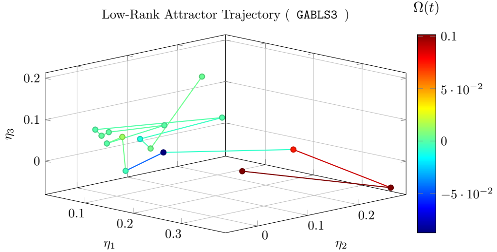
Figure 3: 3D attractor state orbit trajectory. Color variation tracks Attractor Spin (\Omega) , separating shear breakout acceleration (cool blue) from radiative collapse configurations (warm red).
