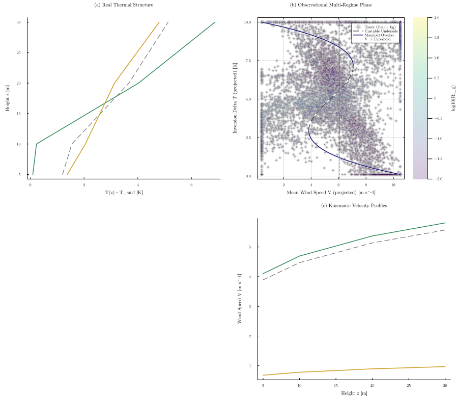
Figure 2: Campaign-resolved real-data aligned profile/scatter diagnostic for CASES-99 . The panel maps reduced manifold coordinates into the operational (\Delta T, V) chart, with side profiles shown in a stripped visual style to emphasize structural alignment rather than plot ornamentation.
