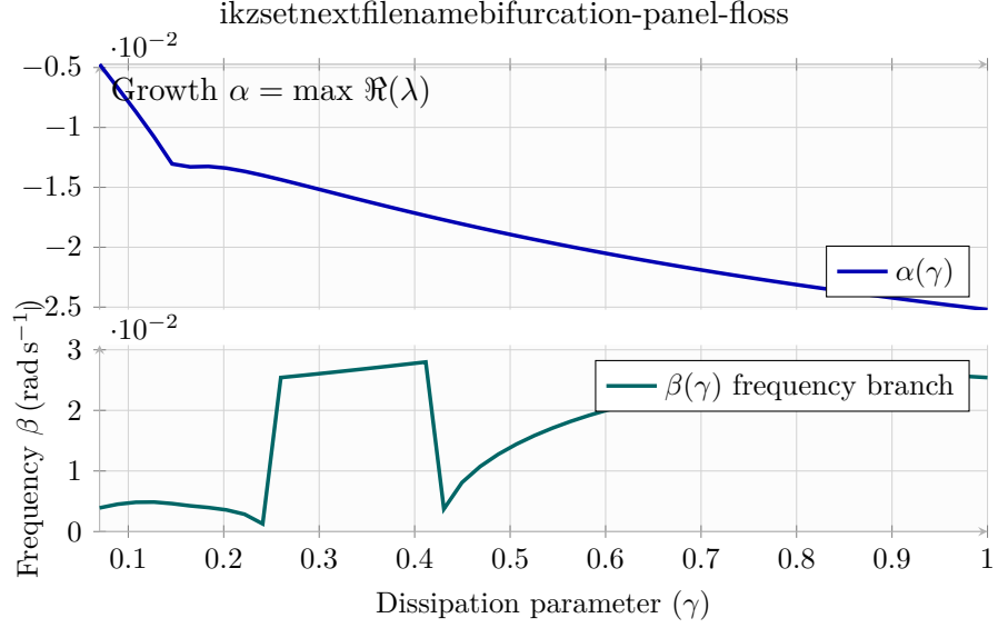
Figure 3: Stage 5 parameter continuation spectrum: the top panel charts the principal manifold stability branch \alpha(\gamma) , while the bottom panel shows the aligned oscillation-frequency branch \beta(\gamma) when available.
