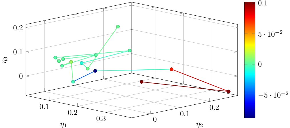
Low-Rank Attractor Trajectory ( GABLS3 )
