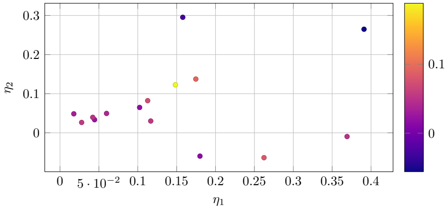
Spectral Orthogonality Projection (GABLS3)
