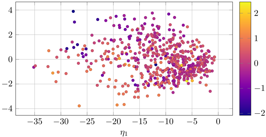
Audit Scatter: BLLAST
