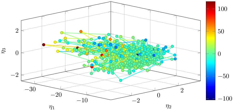
Low-Rank Attractor Trajectory ( BLLAST )
