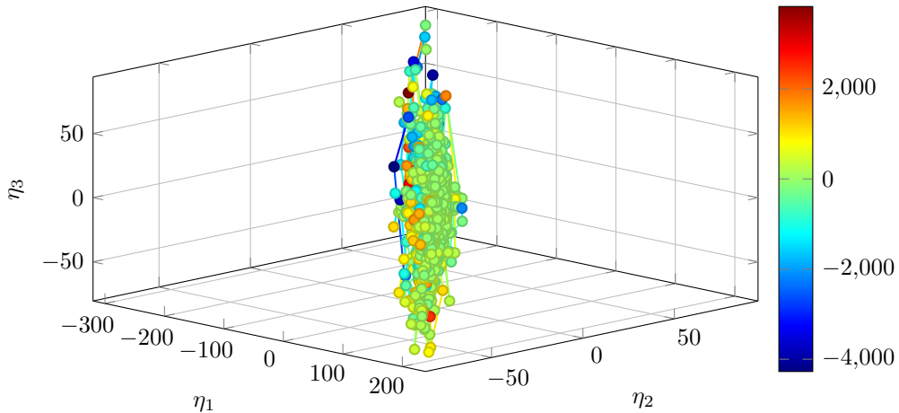
Low-Rank Attractor Trajectory ( FLOSS )
