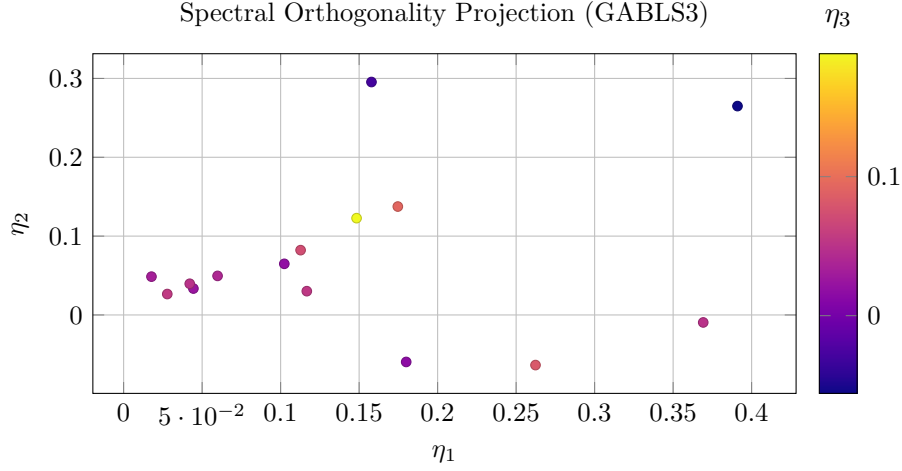
Figure 3: Projected attractor coordinates with orthogonality structure visualized via \eta_3 color encoding.
