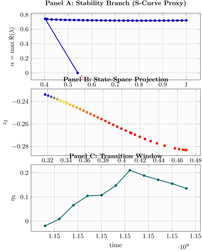
Figure 1: Three-panel transition exhibit. Panel A tracks the stability branch and the Hopf-like crossing. Panel B projects the continuation branch in reduced manifold coordinates. Panel C shows the localized \eta_3 transition window from campaign trajectories.
