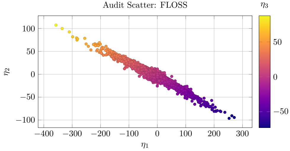
Figure 1: Audit scatter projection with \eta_3 encoded as the color channel.
