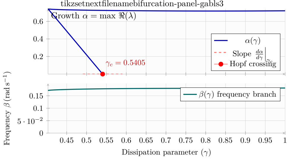
Figure 5: Stage 5 parameter continuation spectrum: the top panel charts the principal manifold stability branch \alpha(\gamma) , while the bottom panel shows the aligned oscillation-frequency branch \beta(\gamma) when available.
