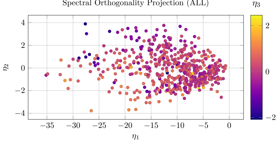
Figure 2: Projected attractor coordinates with orthogonality structure visualized via \eta_3 color encoding.
