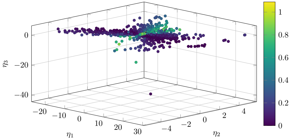
Low-Rank Attractor Trajectory ( CASES-99 )
