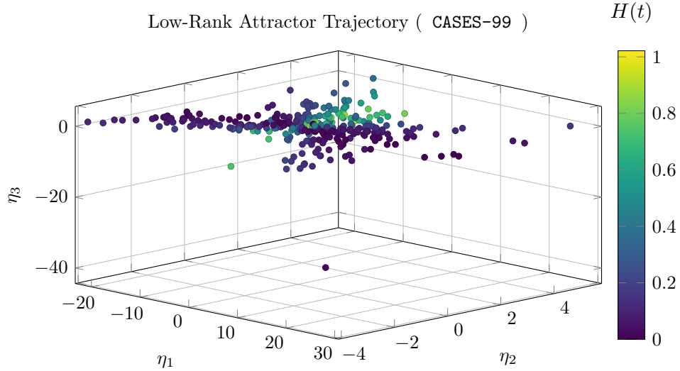
Figure 1: 3D attractor state trajectory colored by singular value entropy.
