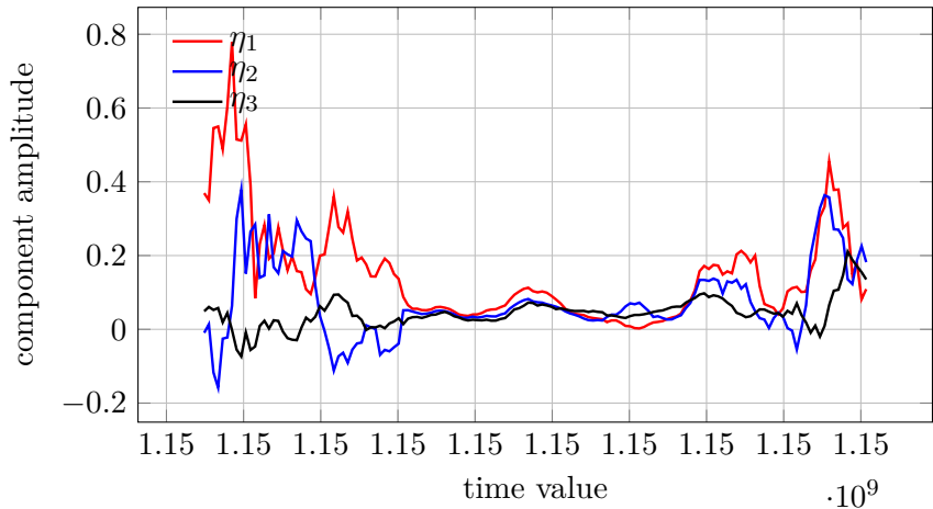
Audit Trajectory Components: GABLS3
