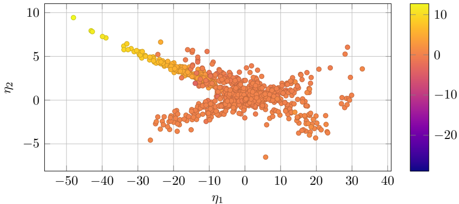
Spectral Orthogonality Projection (ALL)
