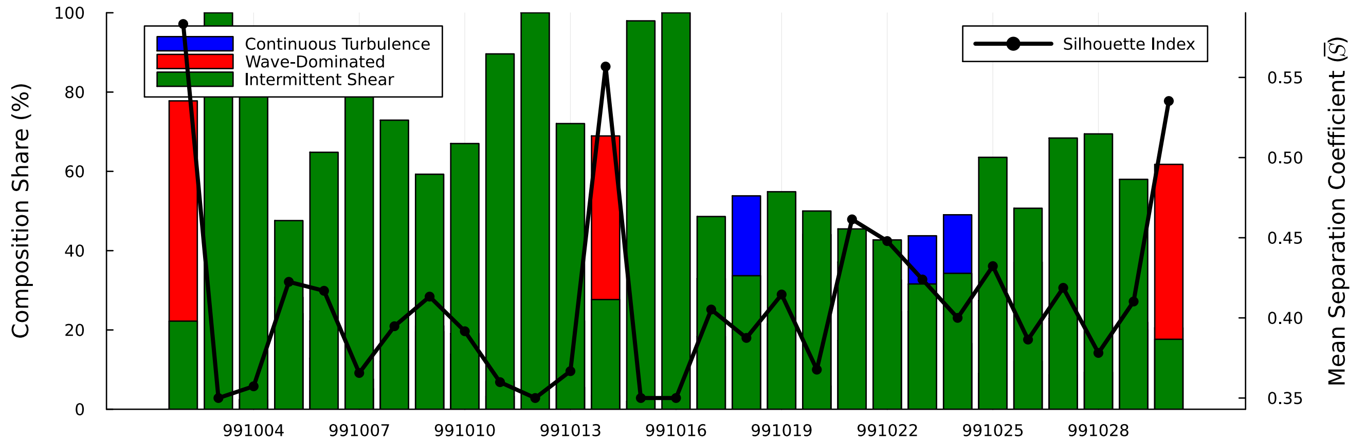
Boundary Layer Regime Composition History
