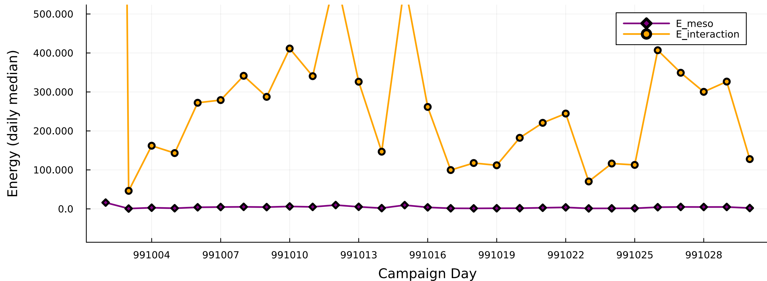
Wave-Turbulence Coupling Energetics
