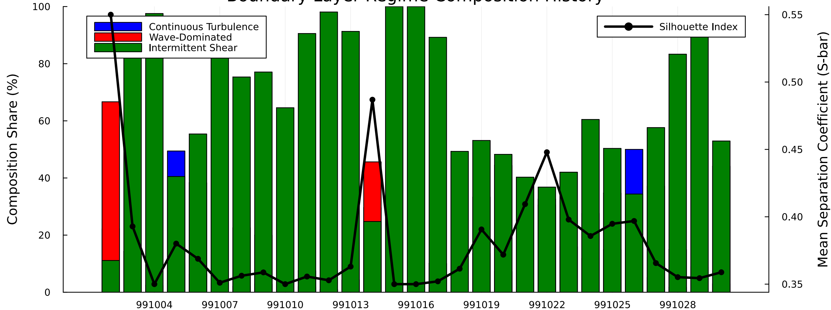
Boundary Layer Regime Composition History
