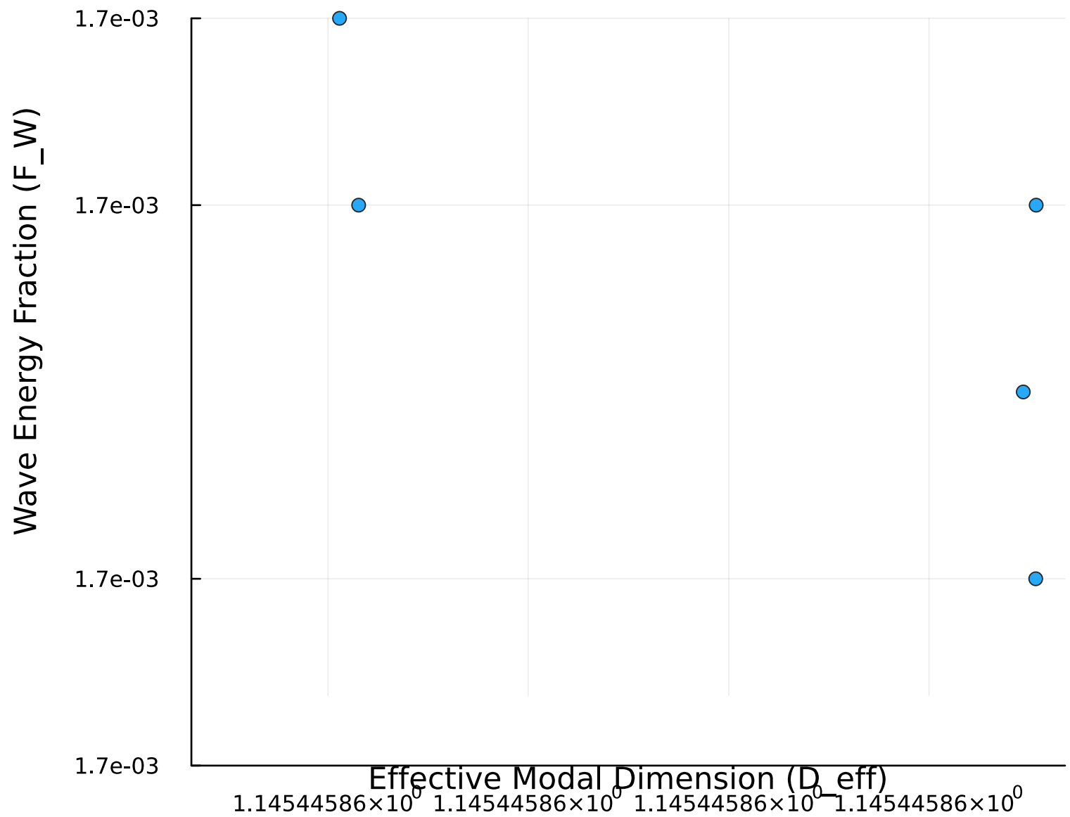
Energy-Dimension Plane [1999-10-03]
