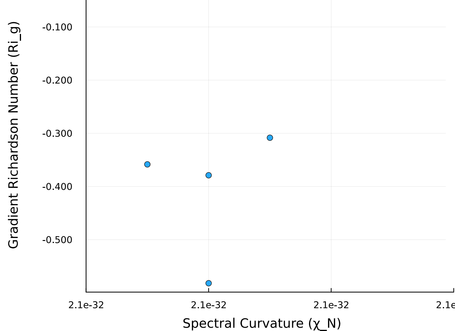
Curvature-Stratification Plane [1999-10-03]
