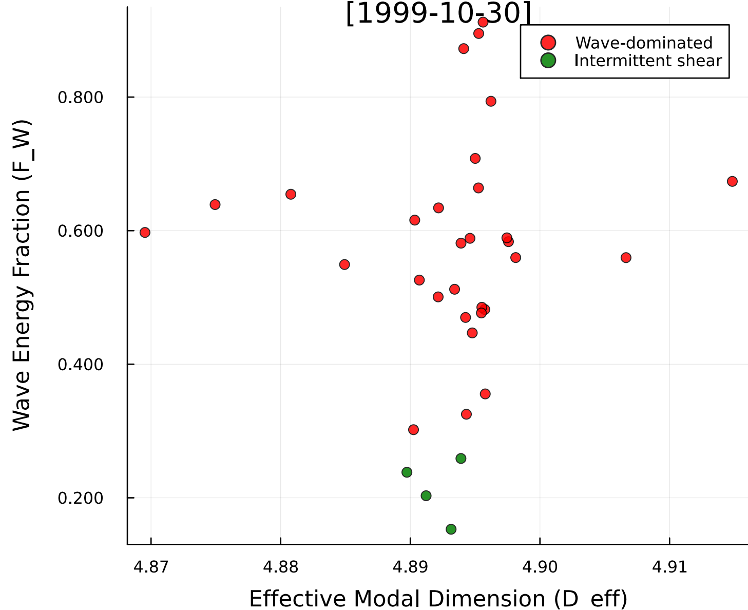
Energy-Dimension Plane
