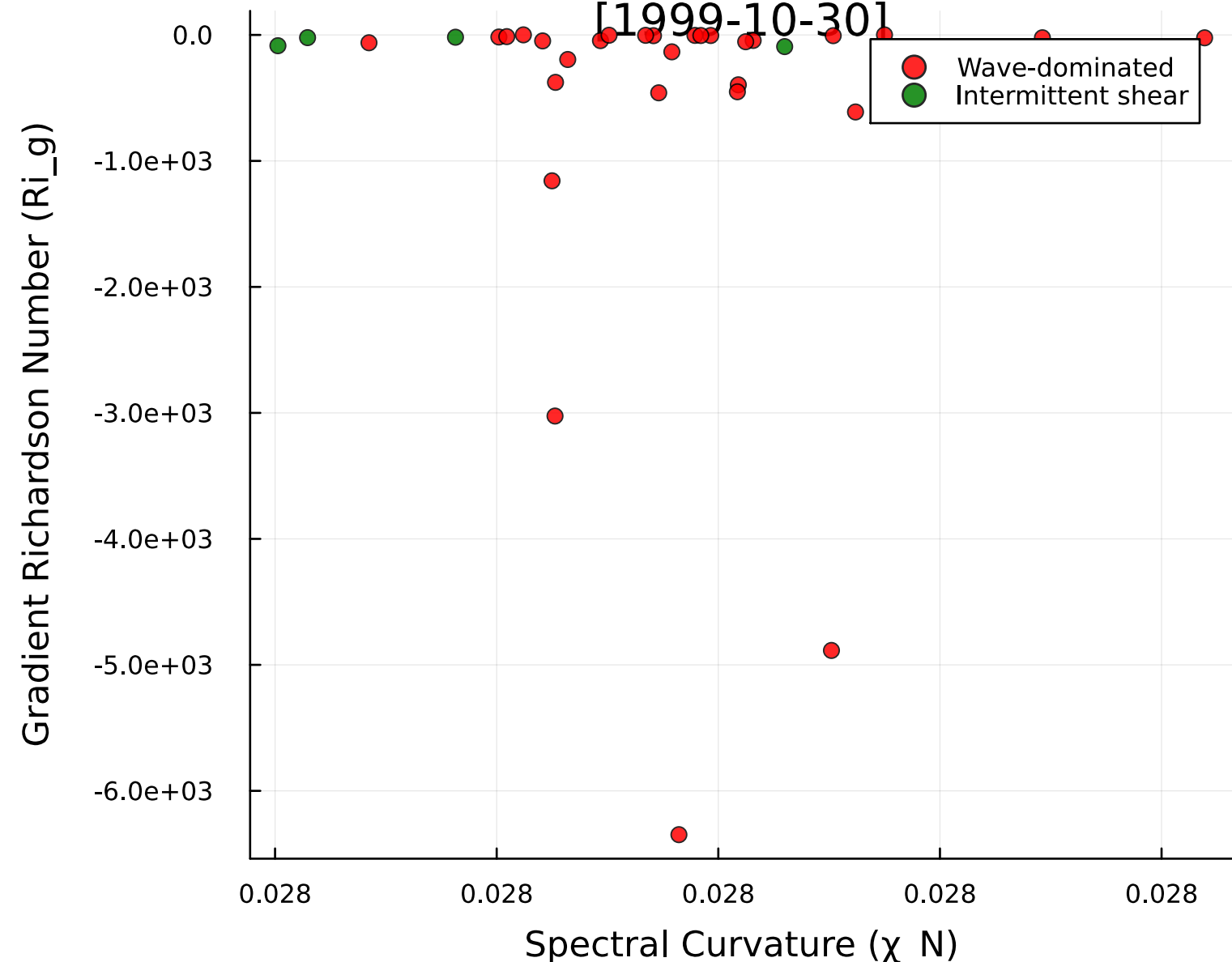
Curvature-Stratification Plane
