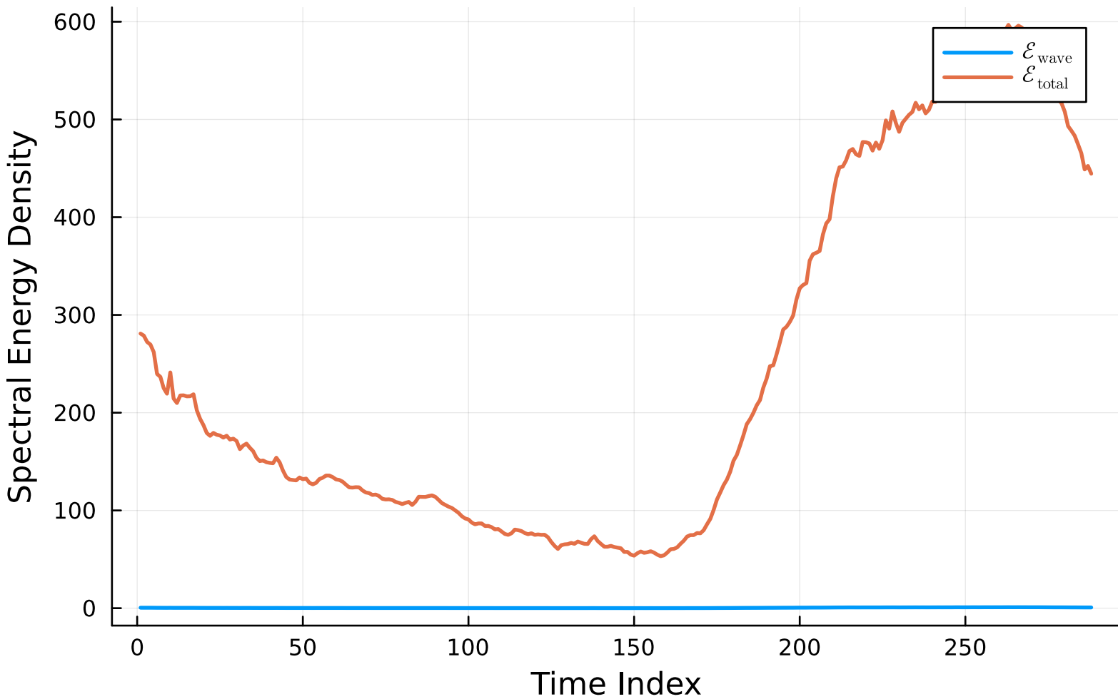
CASES-99 Energy Components (_991021)
