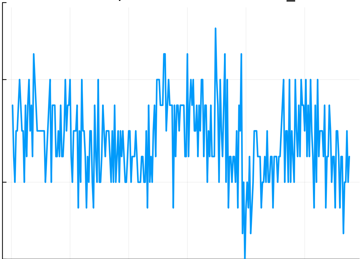
CASES-99 Temporal Feature Trace (_991008)
