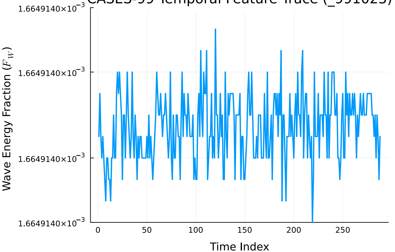
CASES-99 Temporal Feature Trace (_991023)
