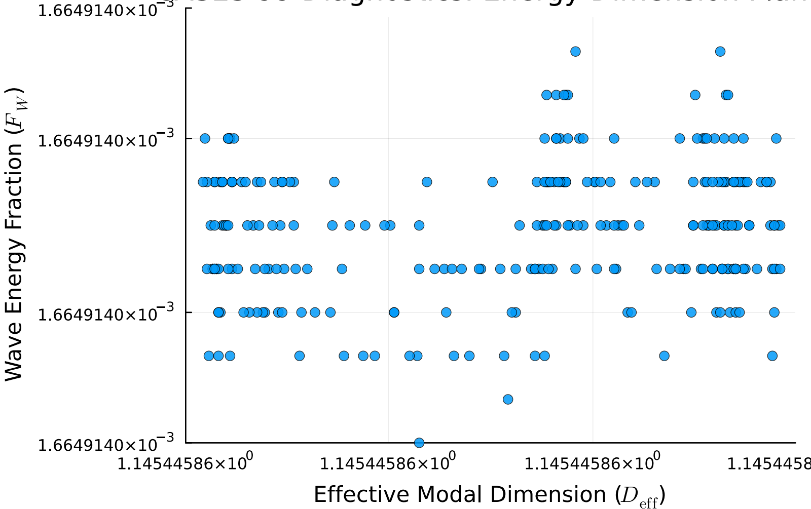
CASES-99 Diagnostics: Energy-Dimension Plan
