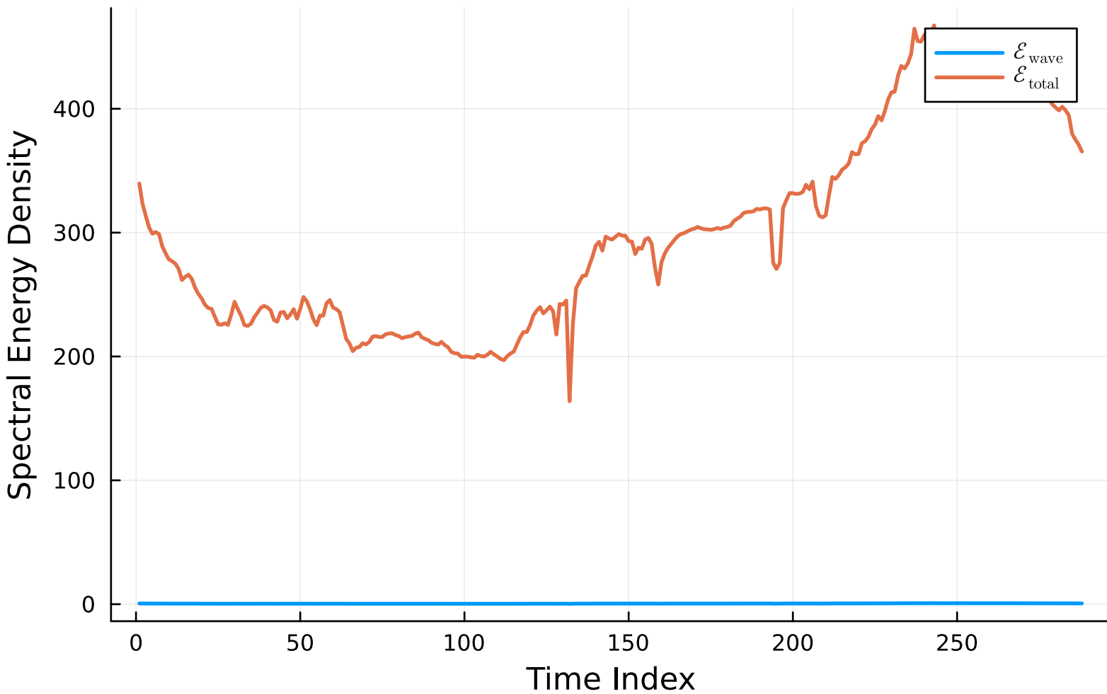
CASES-99 Energy Components (_991008)
