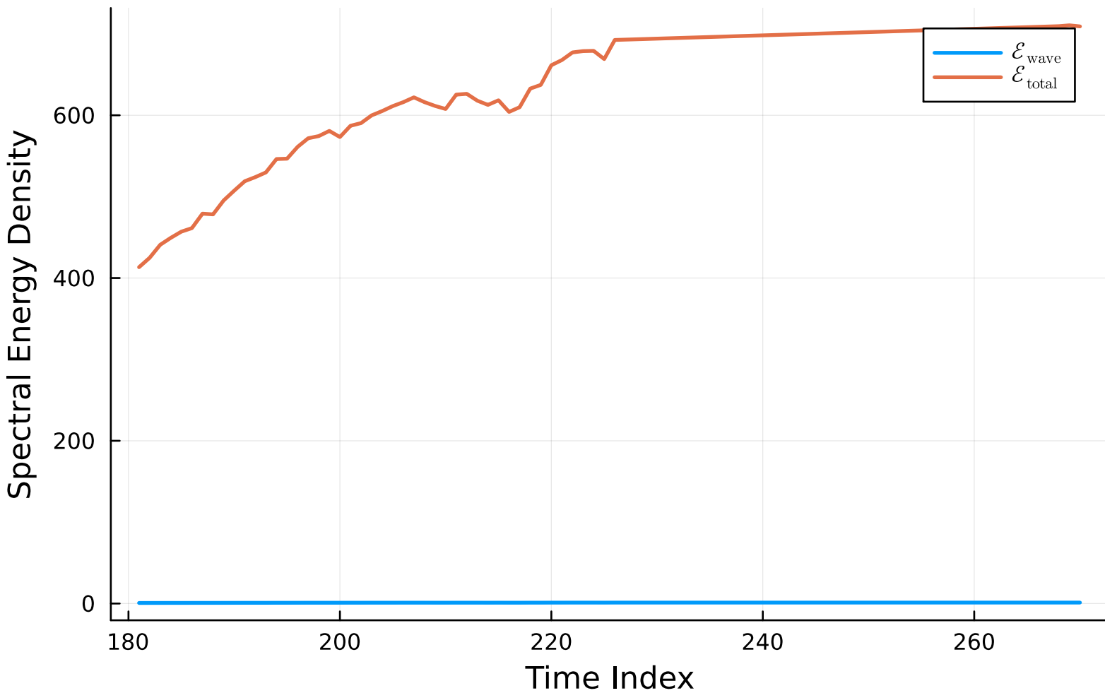
CASES-99 Energy Components (_991015)
