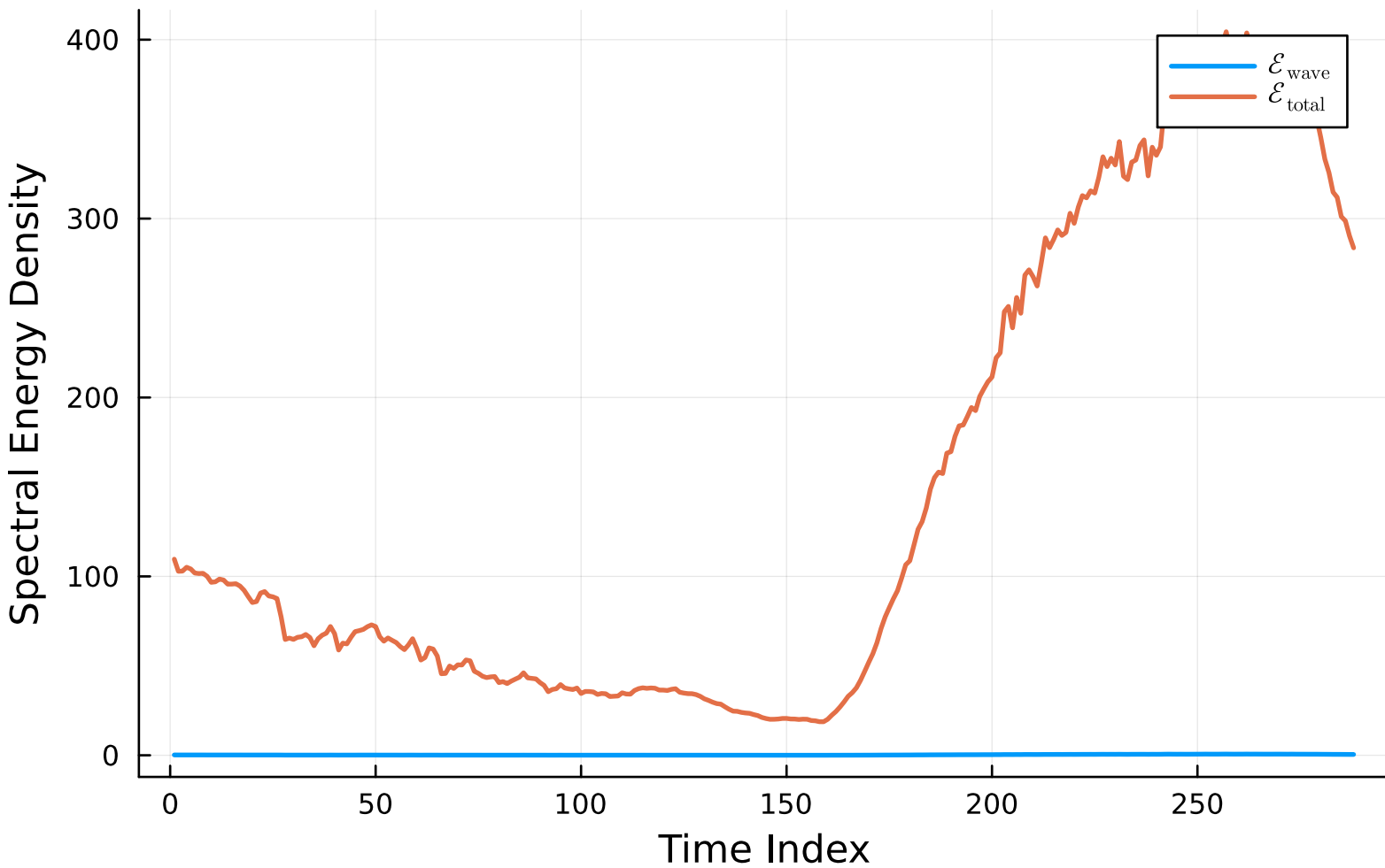
CASES-99 Energy Components (_991020)
