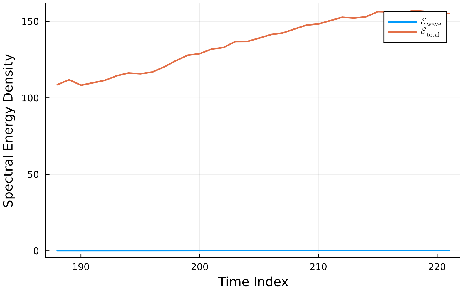
CASES-99 Energy Components (_991030)
