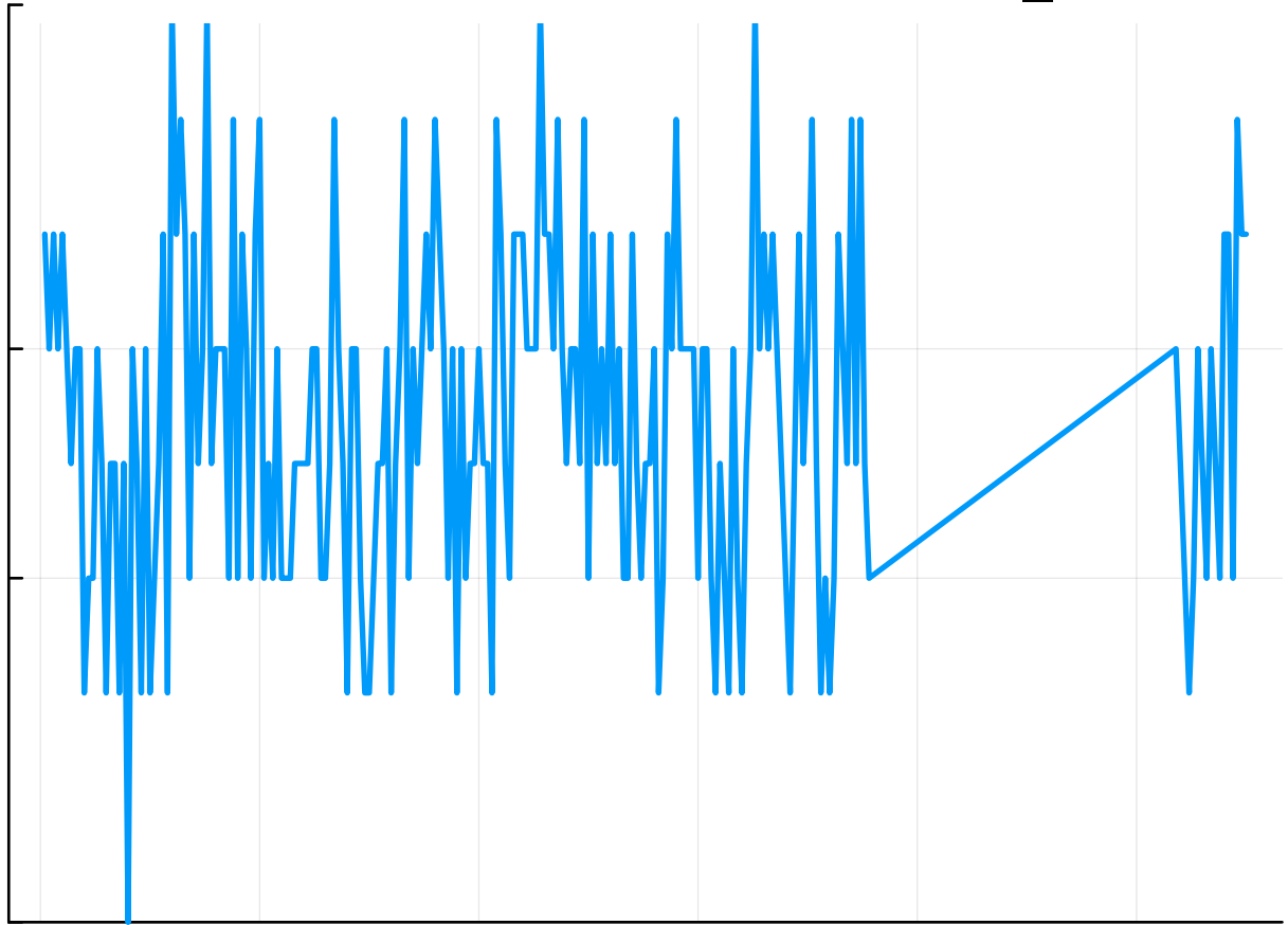
CASES-99 Temporal Feature Trace (_991014)
