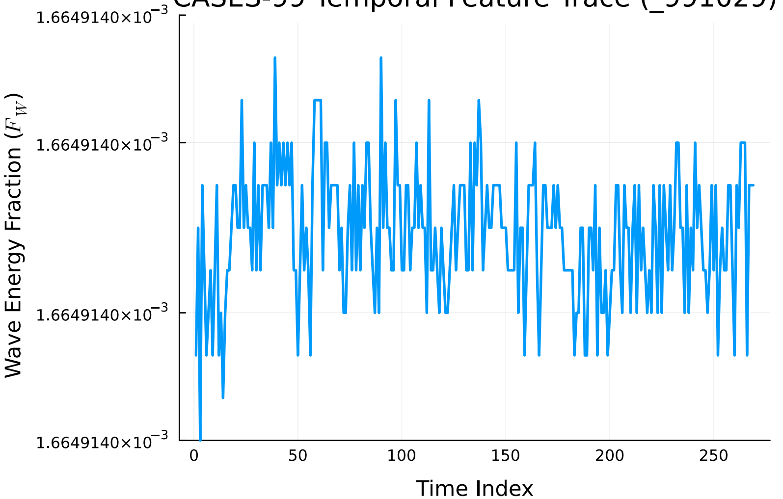
CASES-99 Temporal Feature Trace (_991029)
