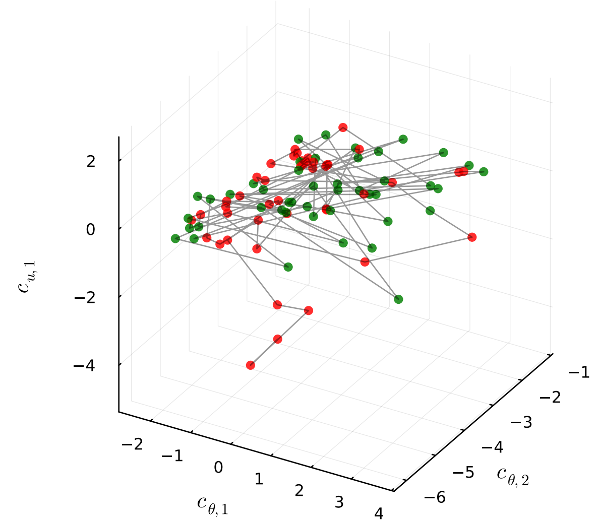
Chebyshev Coefficient-Space Trajectory
