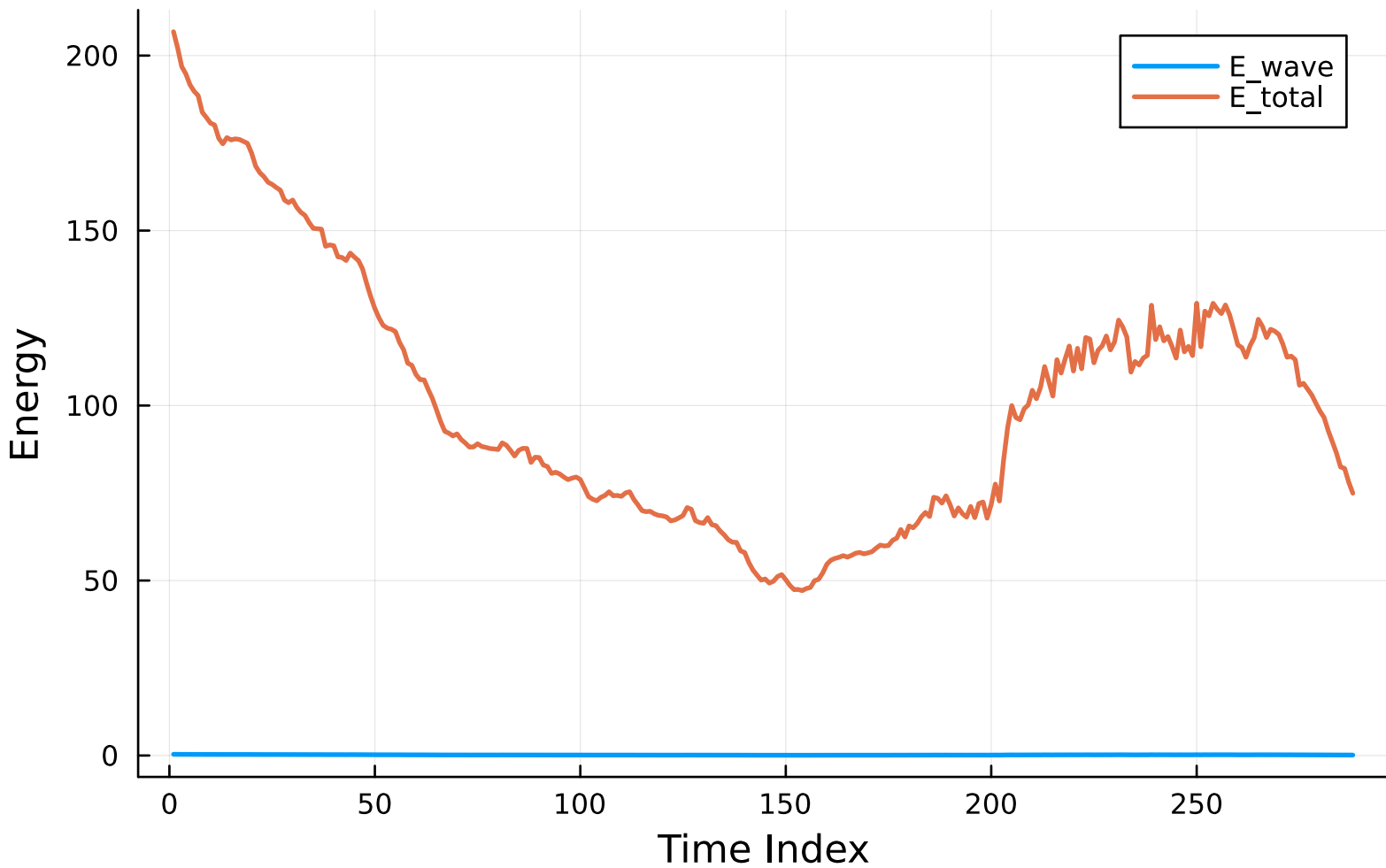
CASES-99 Energy Components (_991017)
