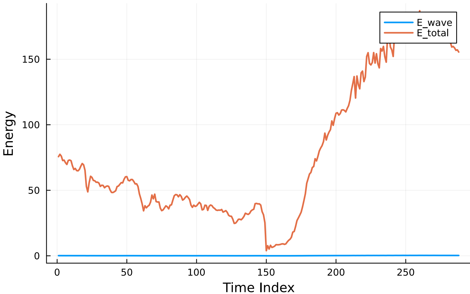
CASES-99 Energy Components (_991018)
