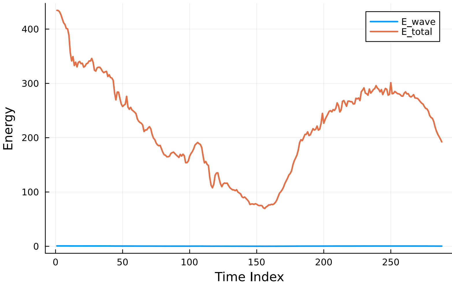
CASES-99 Energy Components (_991022)
