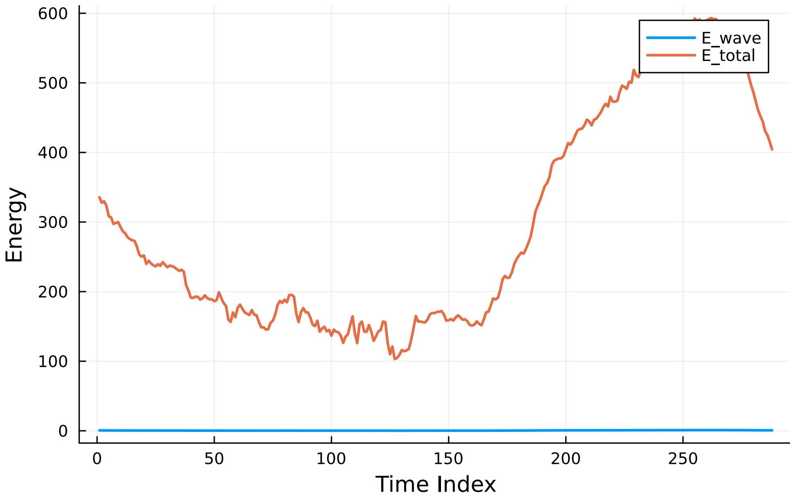
CASES-99 Energy Components (_991026)
