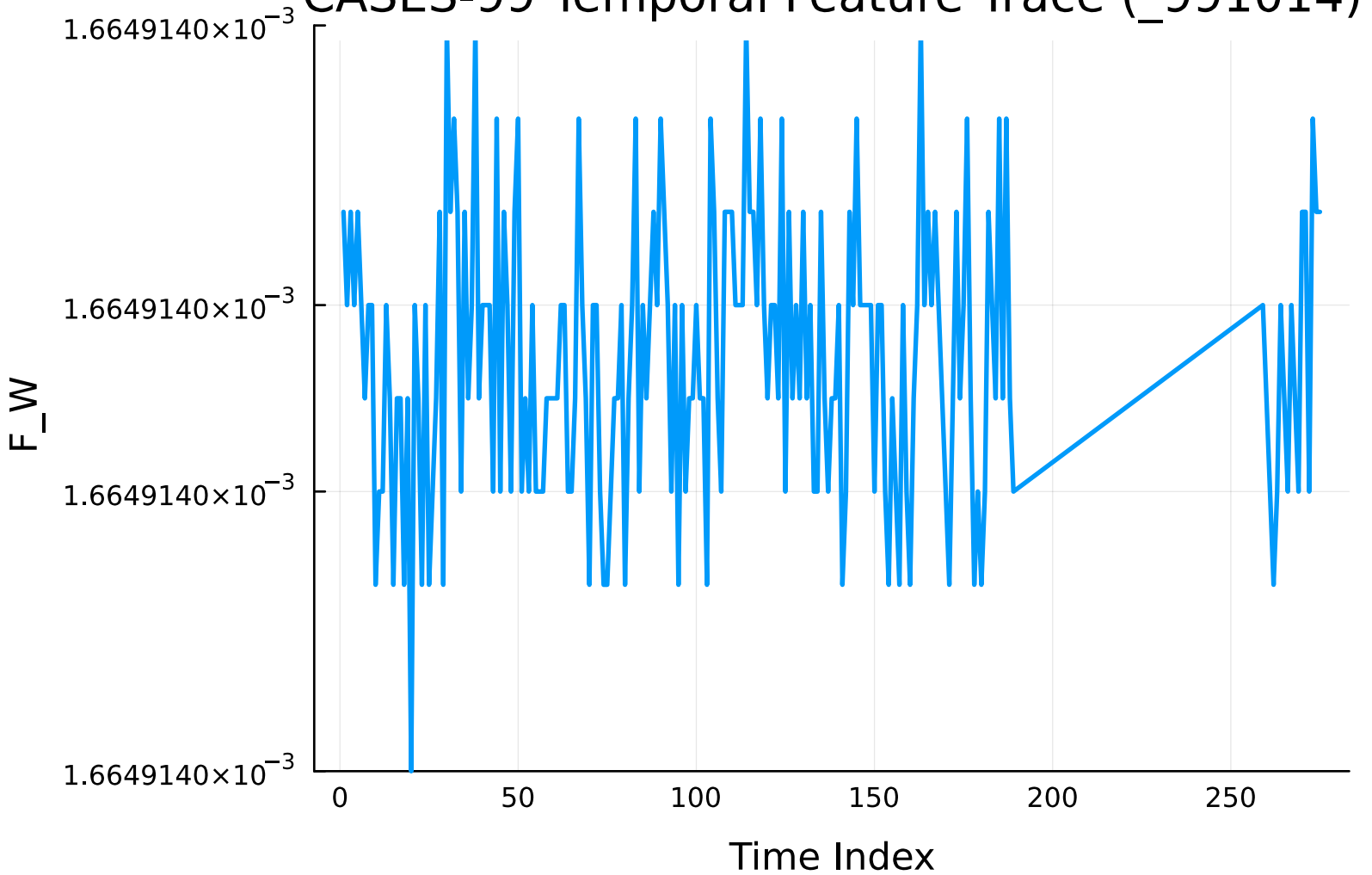
CASES-99 Temporal Feature Trace (_991014)
