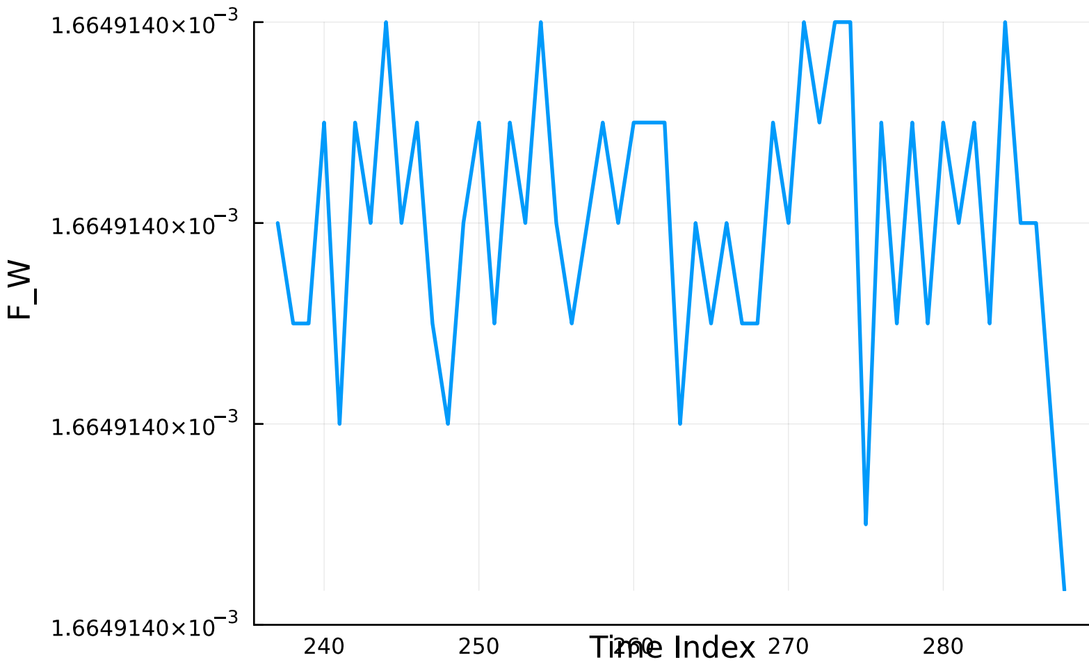
CASES-99 Temporal Feature Trace (_991016)
