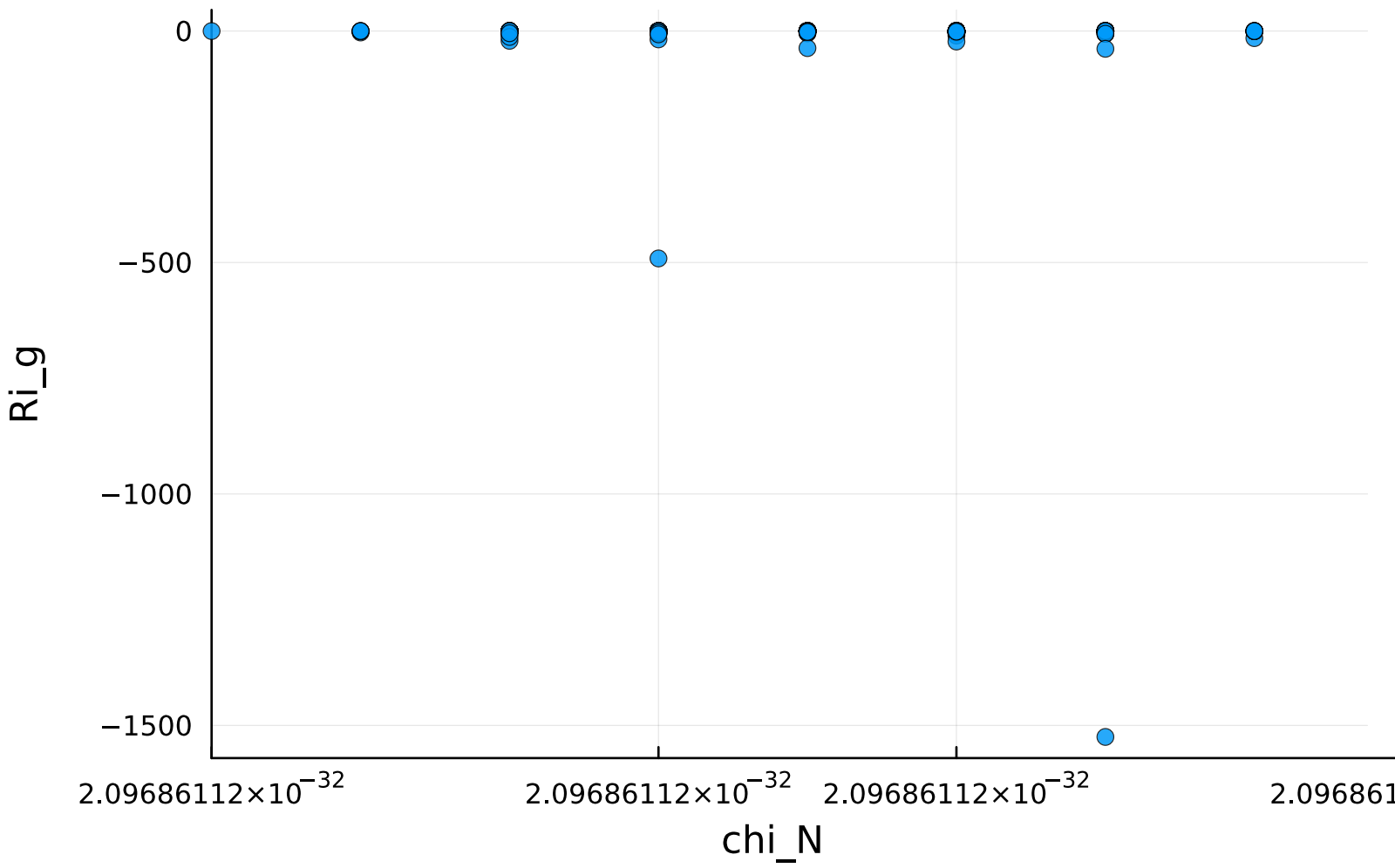
CASES-99 Diagnostics: Curvature-Stratification Plane
